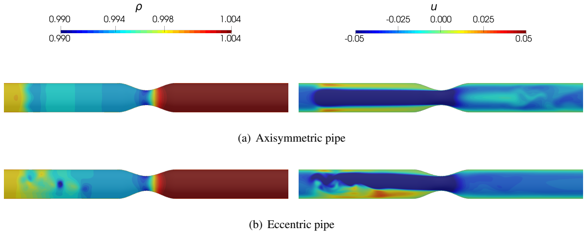
Figure 4: Contours of density and velocity component determined by an axisymmetric and an eccentric stenotic pipe, (a) axisymmetric pipe, (b) eccentric pipe.
